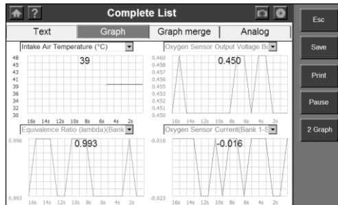
Figure 3.32: Live Data Screen-Graph Display
