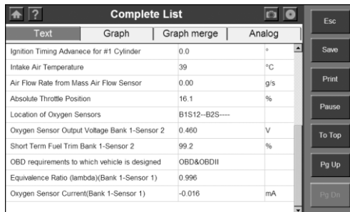
Figure 3.31: Live Data Screen-Digital Display
