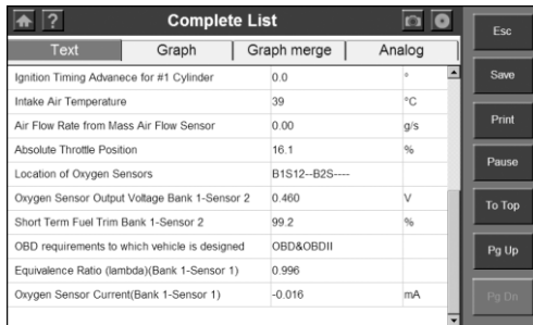
Figure 3.30: Live Data Screen
