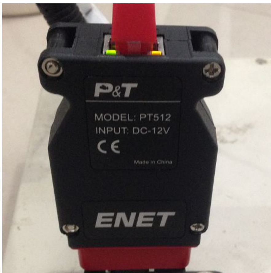
Picture5. Connection mode of ENET
